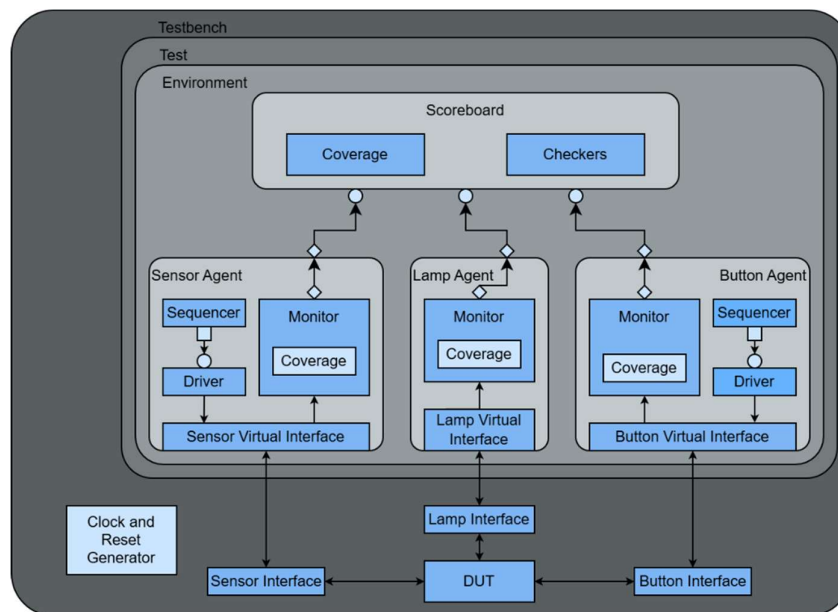
Figure 7. Overview of the components necessary for sending stimuli to the DUT
